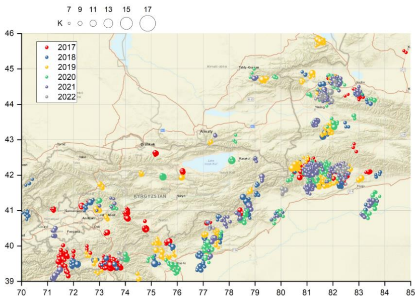
Figure 1 - Map-scheme of earthquake swarms of the seismically active region of study 39^{\circ}-46^{\circ}\text{N} , 70^{\circ}-85^{\circ}\text{E} for 2017-2022 (earthquake swarms in different colors - by years)
