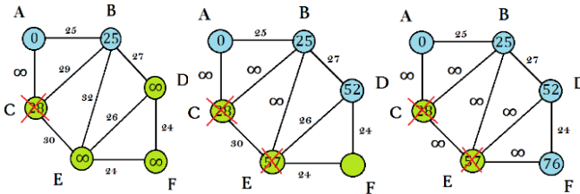
Figure 2. – Further steps of choosing the shortest path
