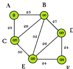
Figure 1. – Network graph
